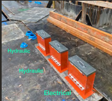
Cast-In Fire Box Installation
